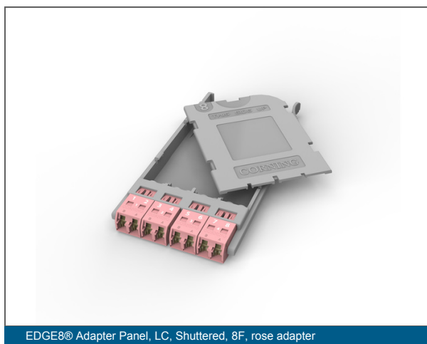
EDGE8® Adapter Panel, LC, Shuttered, 8F, rose adapter
